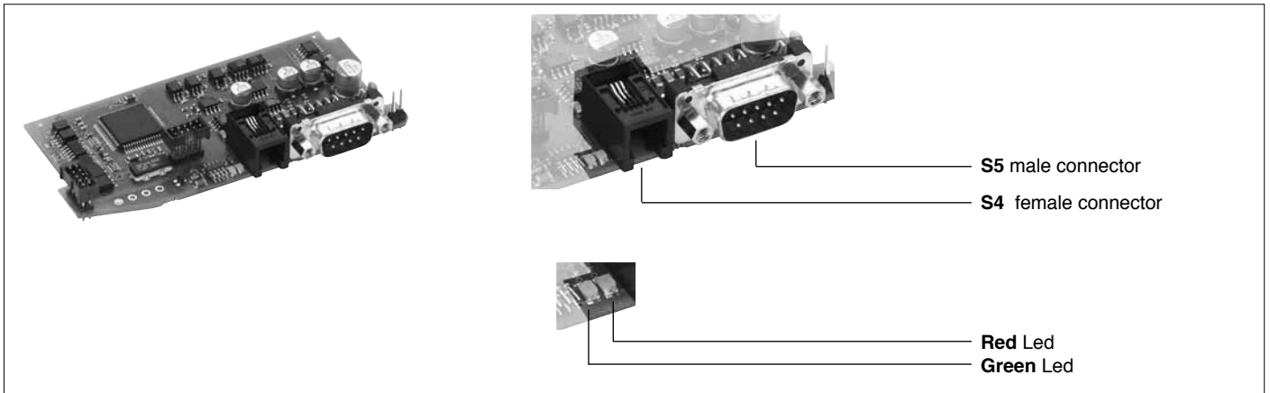
Figure 25 Port2: Fieldbus Modbus RTU/CANOpen Interface
