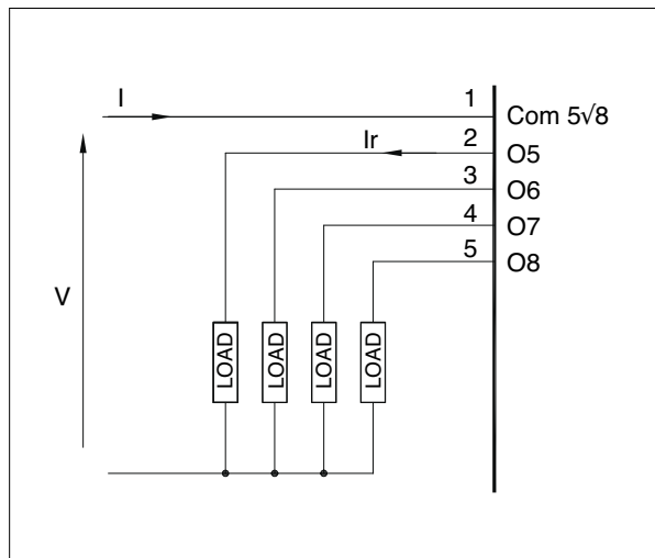
Figure 11 Connection scheme for relay outputs
