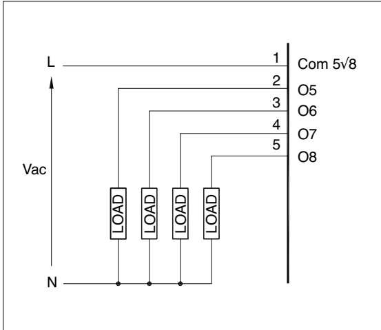
Figure 10 Connection scheme for triac outputs
