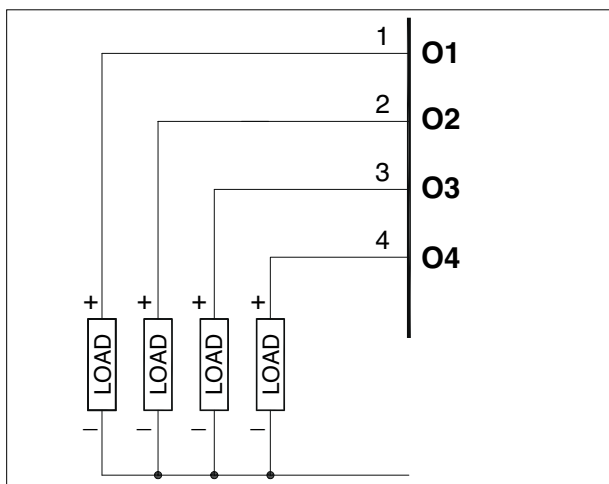
Figure 16 Connection scheme for logic outputs 1...4
