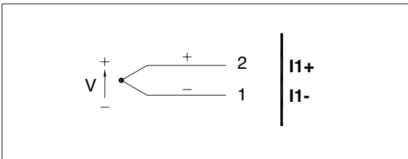
Figure 18 Connection scheme for 60mV TC/linear input
