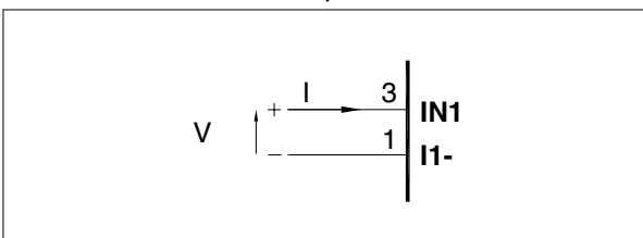
Figure 20 Connection scheme for 1V/20mA linear input
