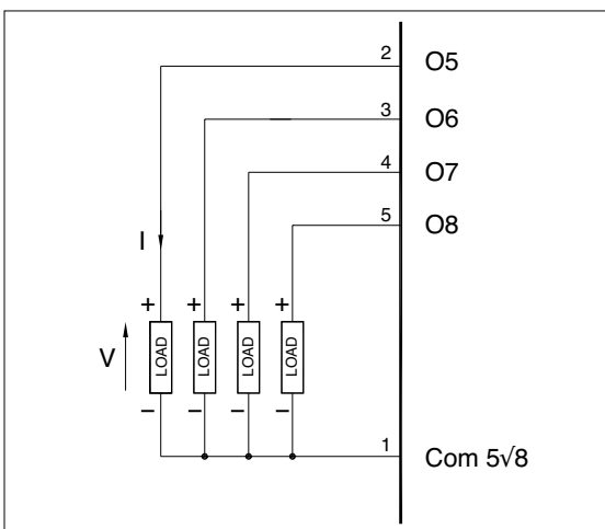
Figure 9 Connection scheme for logic/continuous outputs
