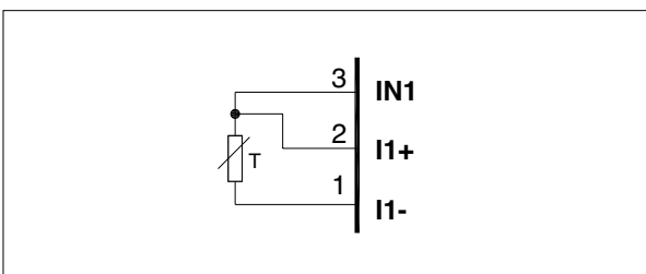
Figure 19 Connection scheme for Pt100 input
