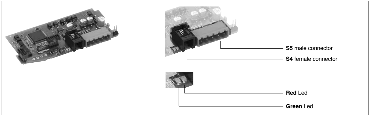
Figure 26 Port2: Fieldbus Modbus RTU/DeviceNet Interface
