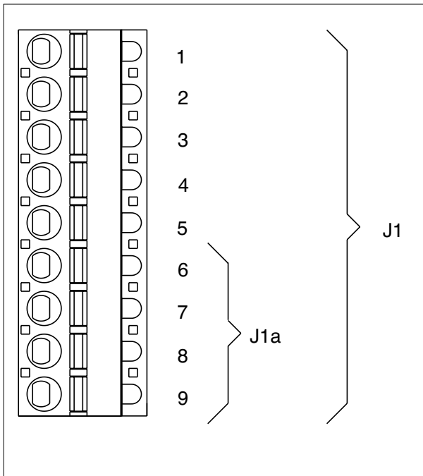
Figure 8 Connector J1
