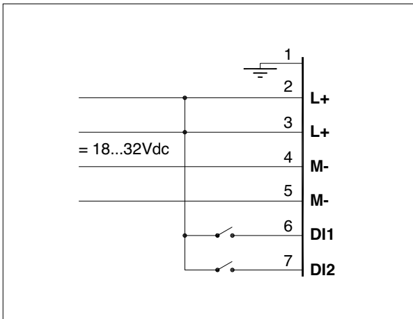
Figure 14 Connection scheme for digital inputs and power supply
