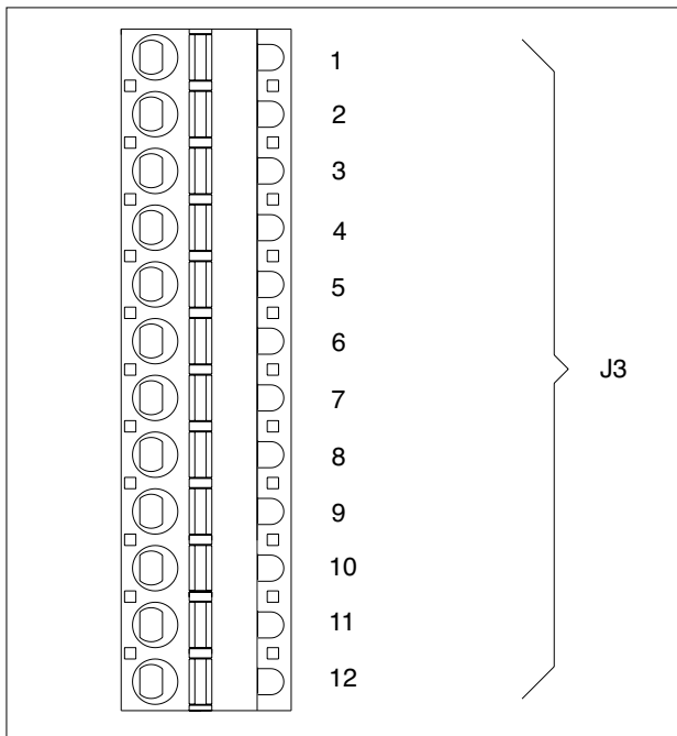
Figure 16 Connection scheme for logic outputs 1...4
