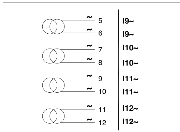
Figure 16b Connection scheme for CT inputs
