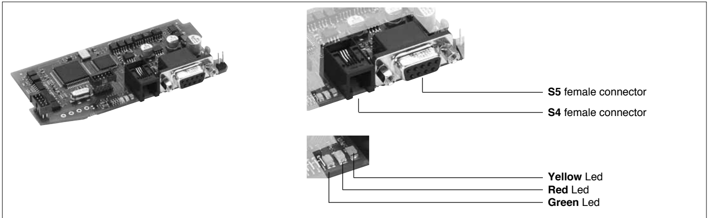
Figure 24 Port2: Fieldbus Modbus RTU/Profibus DP Interface
