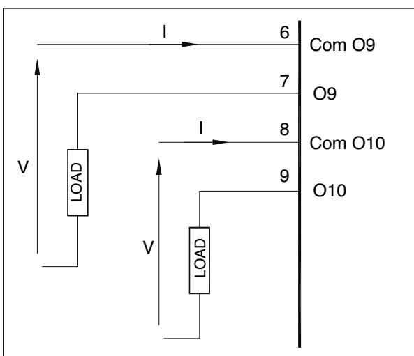
Figure 12 Connection scheme for relay outputs
