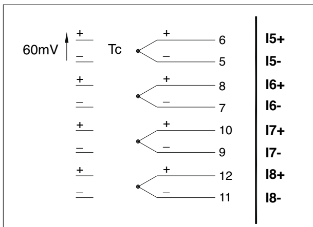
Figure 16a Connection scheme for 60mV/TC auxiliary linear inputs
