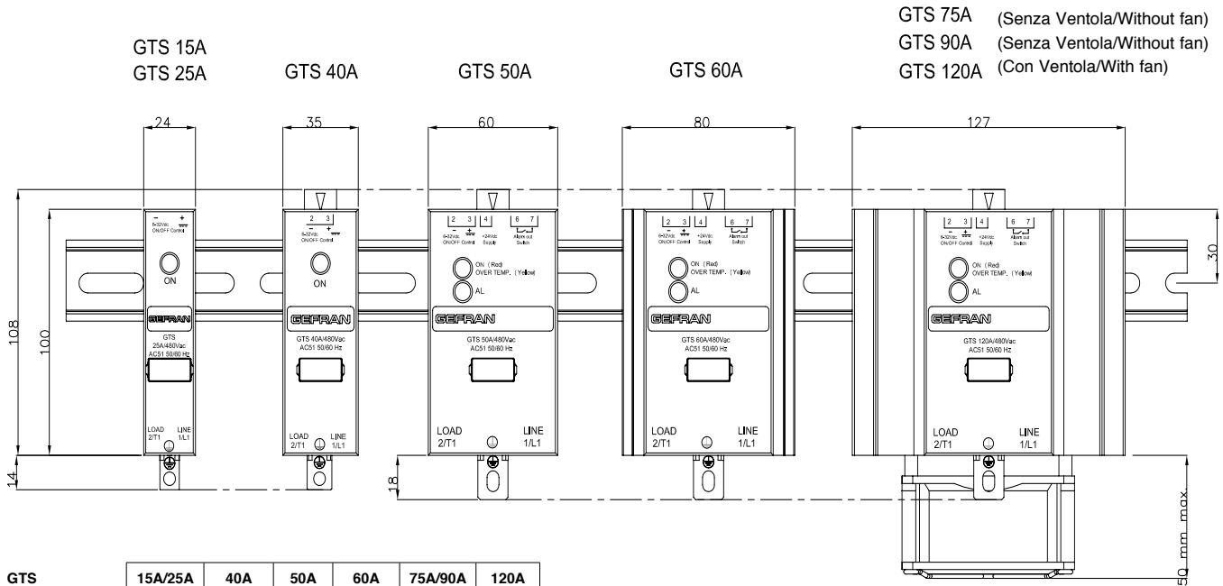
Figure 1 - DIMENSIONS
